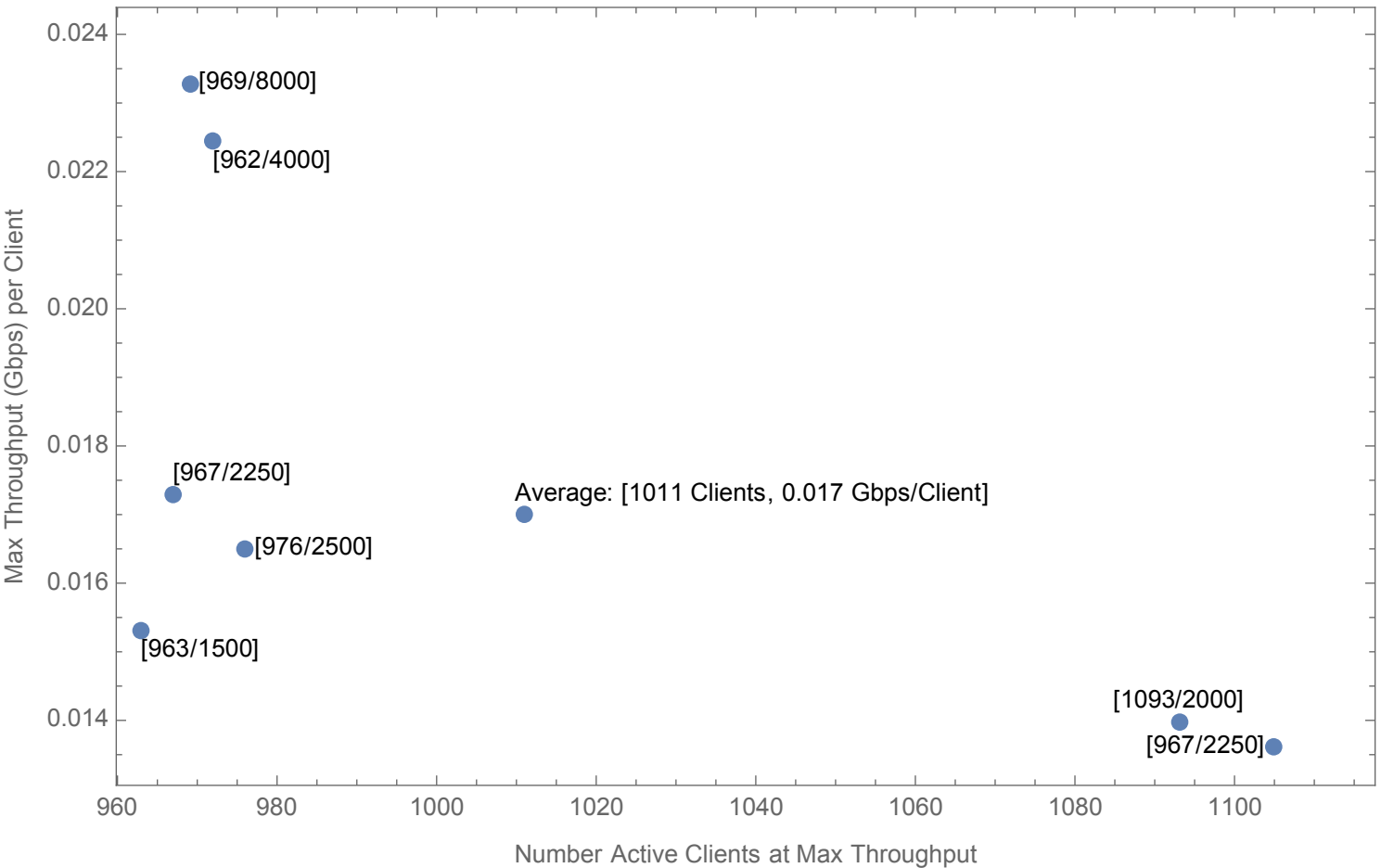
Max Throughput/Client vs Number Active Clients Each Point: [Active Clients/Total Number of Clients Queued] Sleep Time between gfaI-copy instances: 2 seconds
