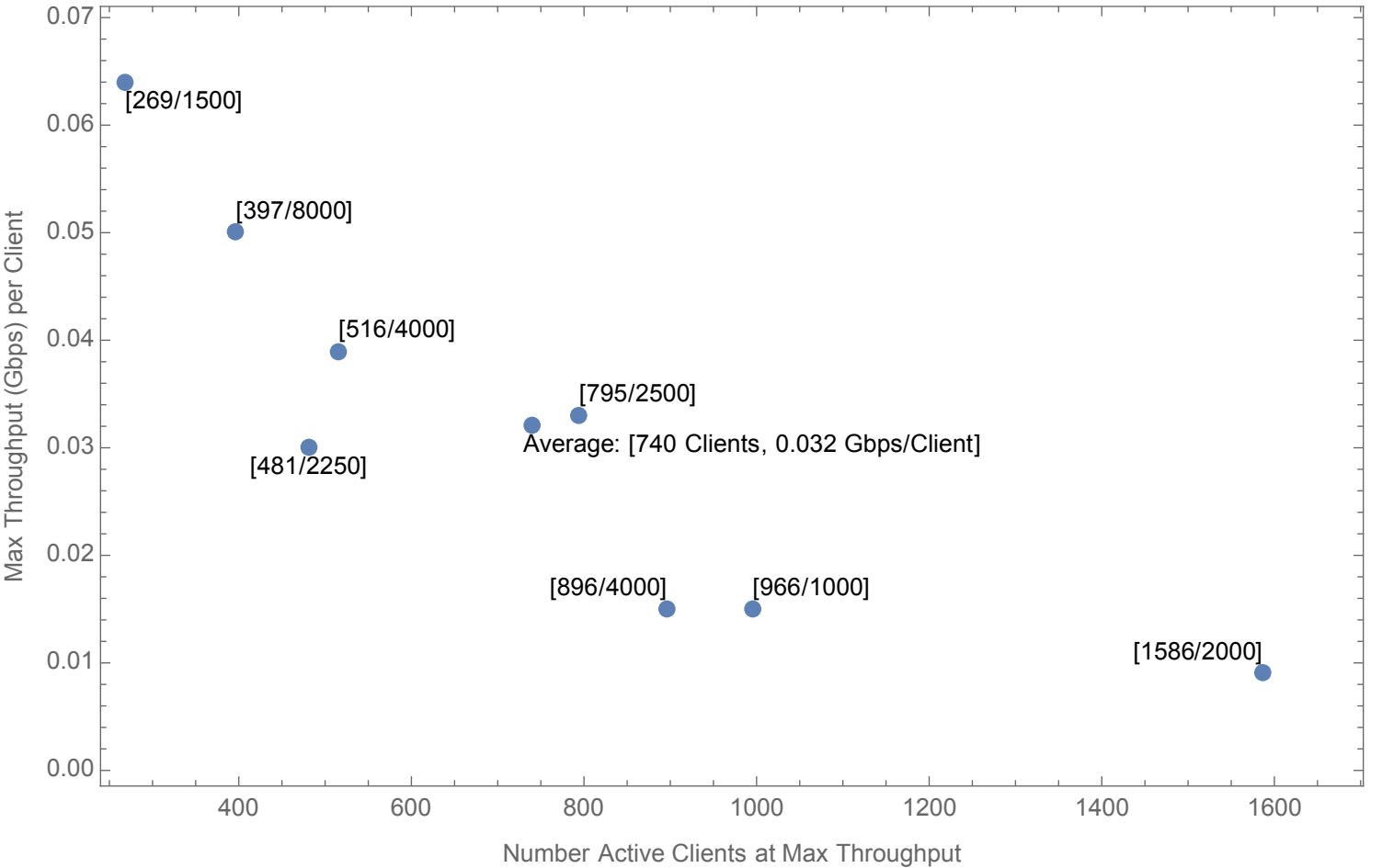
Max Throughput/Client vs Number Active Clients Each Point: [Active Clients/Total Number of Clients Queued] Sleep Time between gfaI-copy instances: 10 seconds
