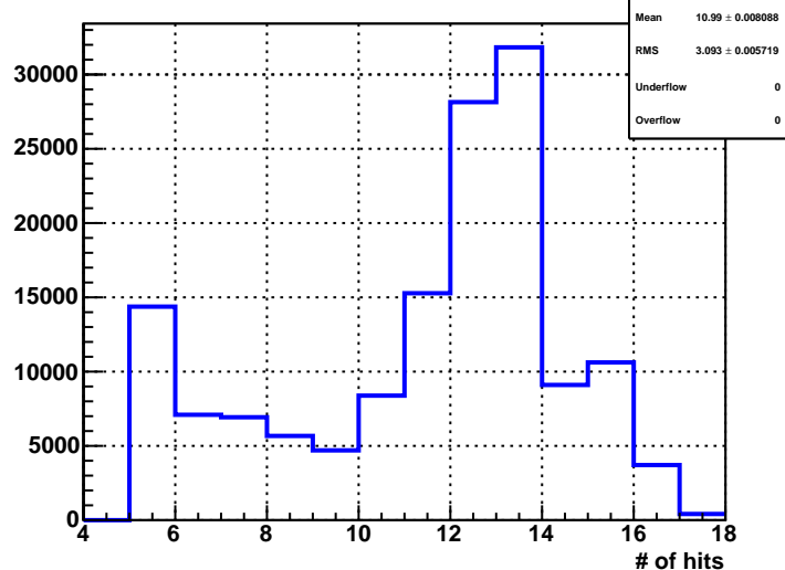
Number of Valid Hits of RecoTrack
