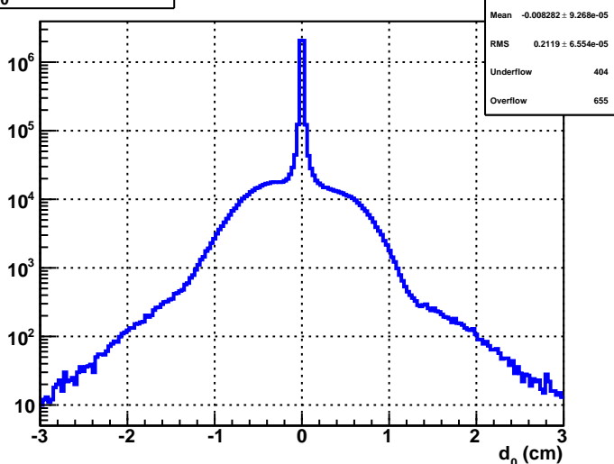
d_0 of RecoTrack
