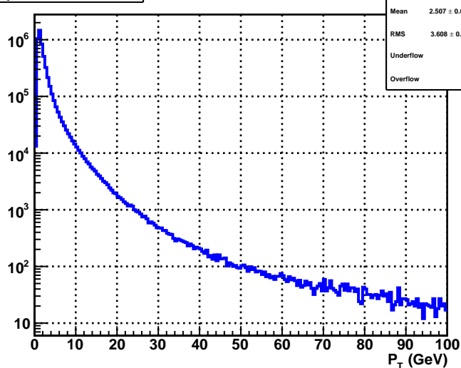
P_T of RecoTrack
