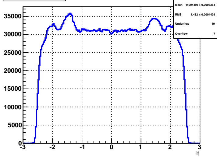
\eta of RecoTrack
