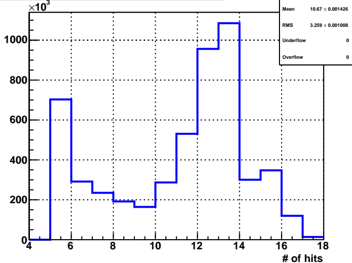
Number of Valid Hits of RecoTrack
