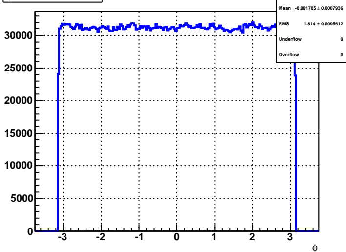
\phi of RecoTrack
