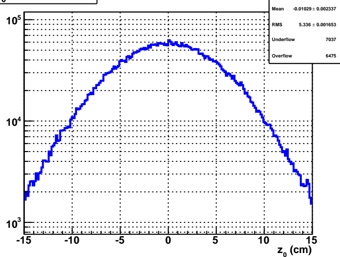
z_0 of RecoTrack
