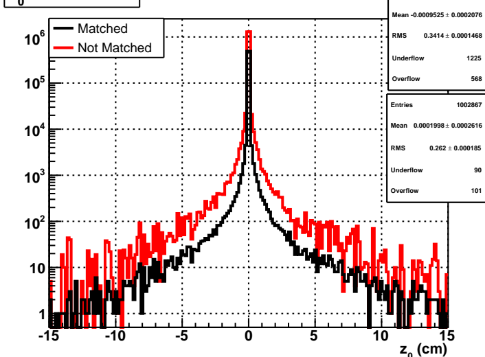
z_0 of SimTrack
