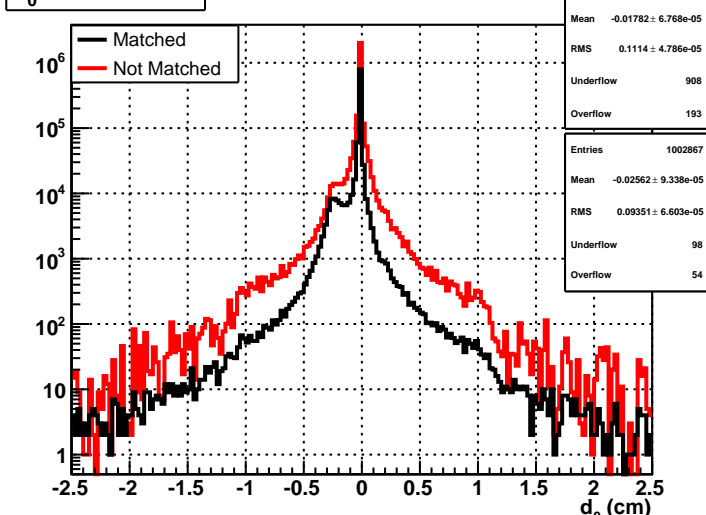
d_0 of SimTrack
