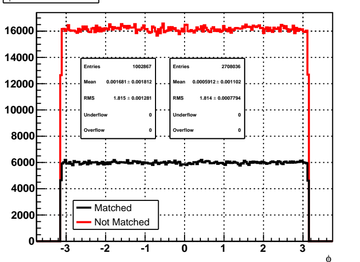
\phi of SimTrack
