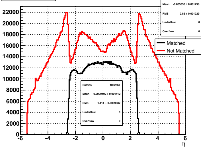
\eta of SimTrack
