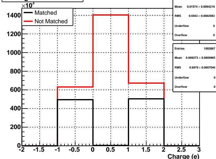
Charge of SimTrack
