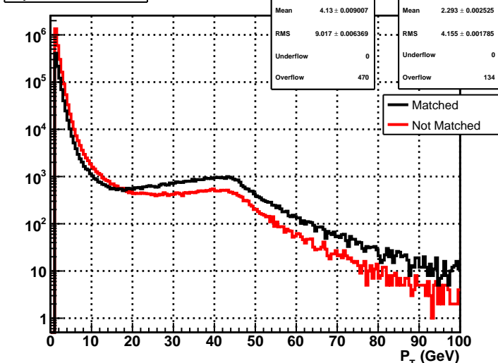
P_T of SimTrack
