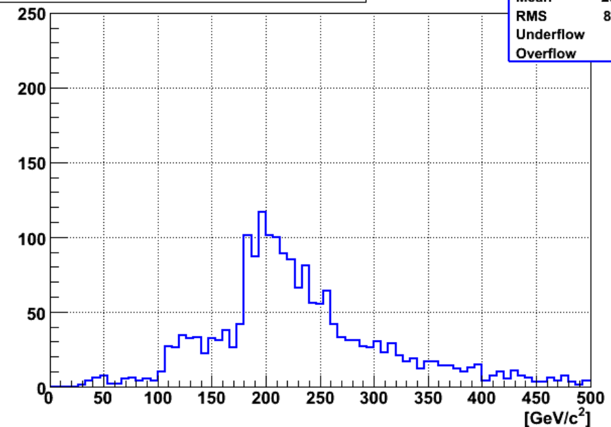
Higgs Candidate ( M_{4l} ) (PPZZ4e_5k)
