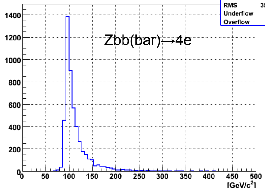
Higgs Candidate ( M_{4l} ) (ZBBbar4e_5k)
