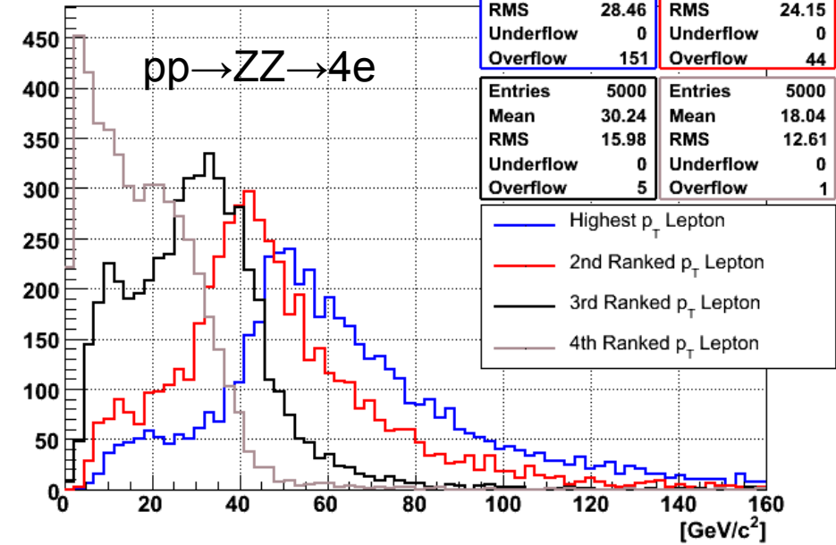
p_T of Lepton (PPZZ4e_5k)
