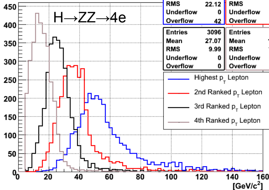
p_T of Lepton (HZZ4e_150_5k)
