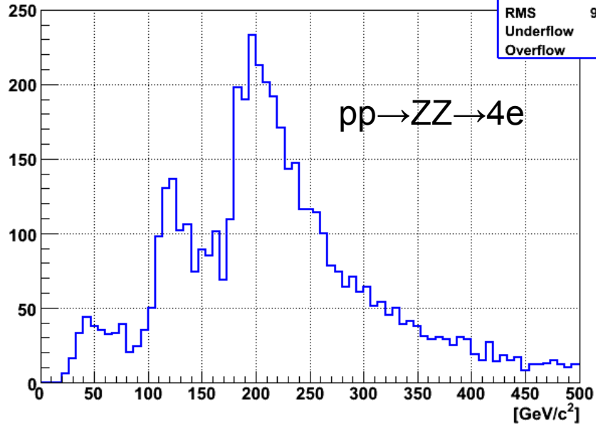
Higgs Candidate ( M_{4l} ) (PPZZ4e_5k)
