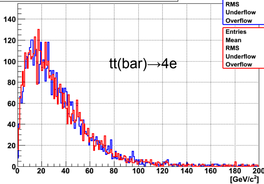
Z Candidate ( M_{l_1l_4} and M_{l_2l_3} ) (TTbar4e_5k)
