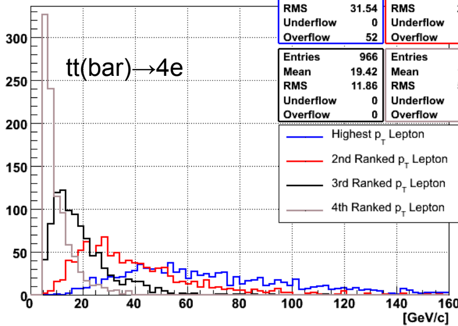
p_T of Lepton (TTbar4e_5k)
