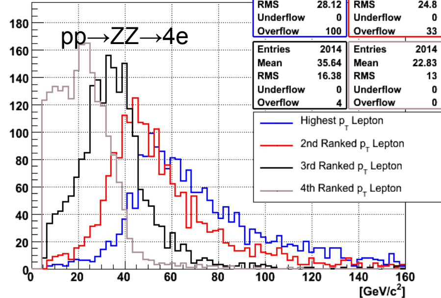
p_T of Lepton (PPZZ4e_5k)
