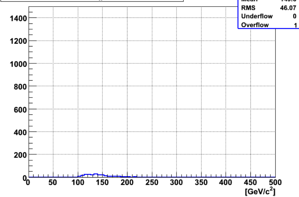
Higgs Candidate ( M_{4l} ) (ZBBbar4e_5k)
