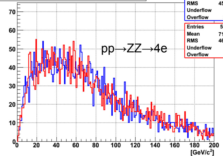
Z Candidate ( M_{l_1l_4} and M_{l_2l_3} ) (PPZZ4e_5k)
