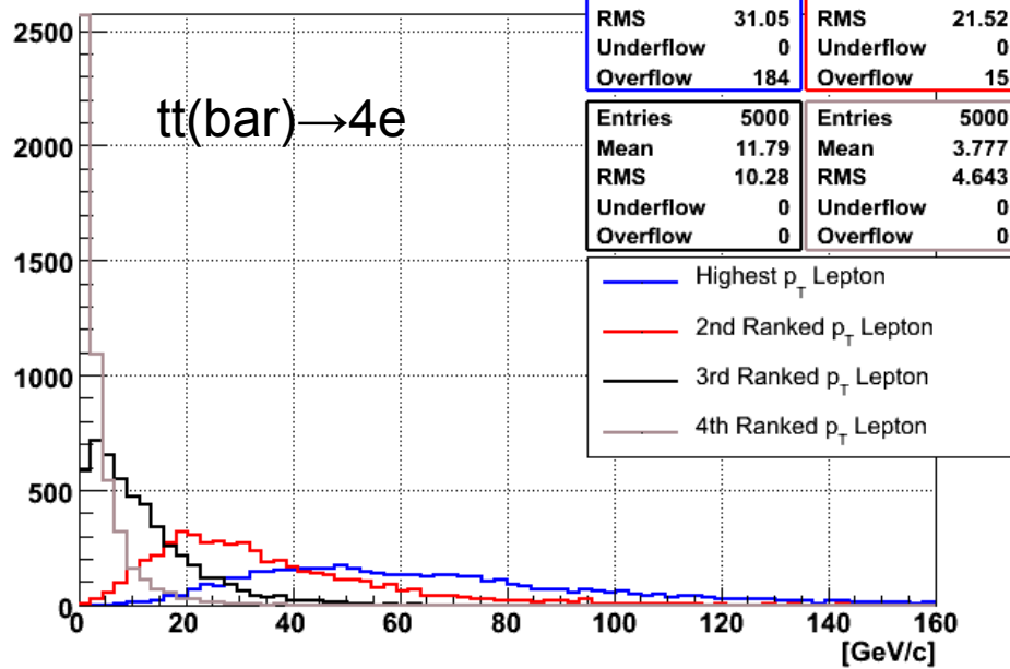
p_T of Lepton (TTbar4e_5k)
