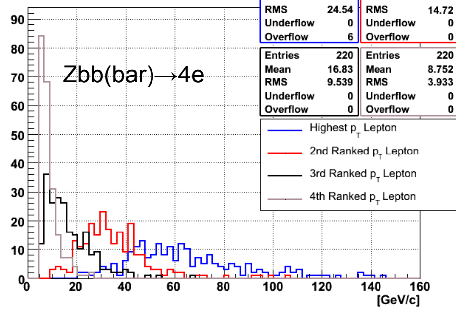
p_T of Lepton (ZBBbar4e_5k)
