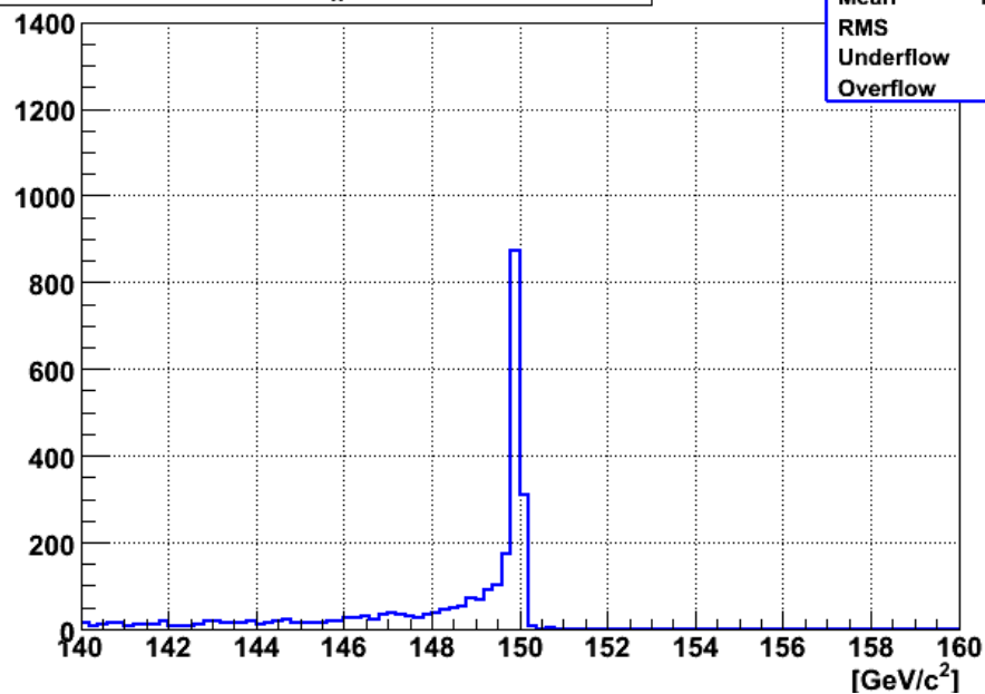
Higgs Candidate ( M_{4l} ) (HZZ4e_150_5k)
