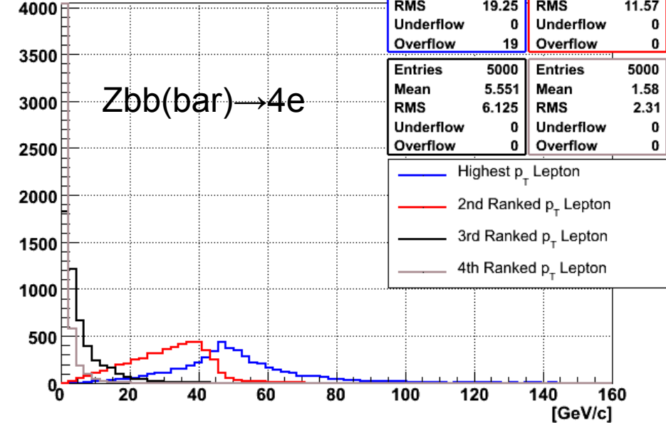
p_T of Lepton (ZBBbar4e_5k)
