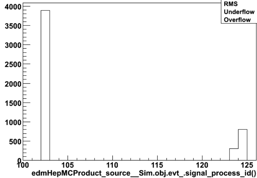
edmHepMCProduct_source_Sim.obj.evt_signal_process_id()
