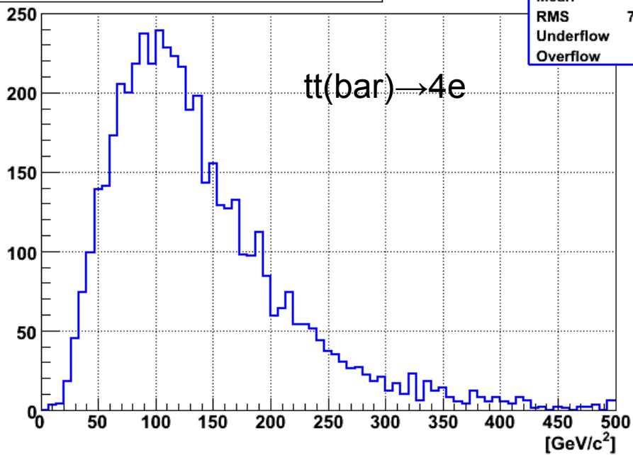
Higgs Candidate ( M_{4l} ) (TTbar4e_5k)
