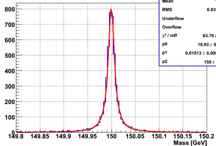
M_{\text{Higgs}} (Generated) (HZZ4e_150_5k)
