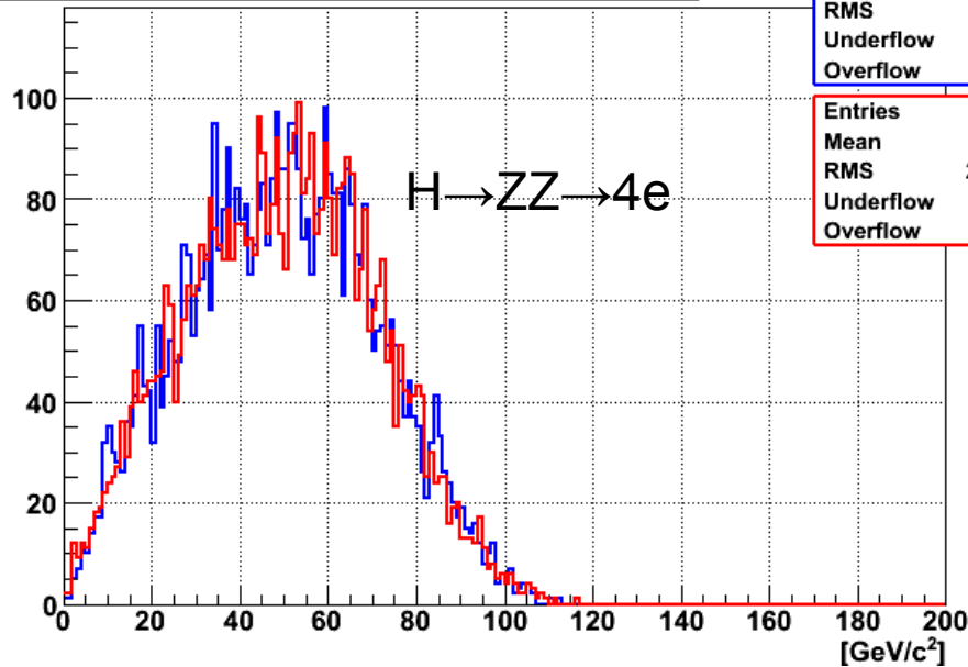
Z Candidate ( M_{l_1l_4} and M_{l_2l_3} ) (HZZ4e_150_5k)
