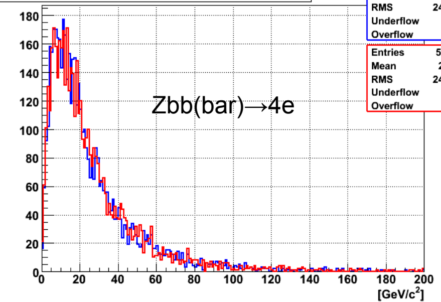
Z Candidate ( M_{l_1l_4} and M_{l_2l_3} ) (ZBBbar4e_5k)
