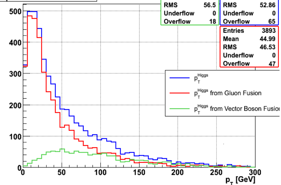
p_{\text{T}}^{\text{higgs}} (HZZ4e_150_5k)
